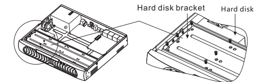
Figure 3-1 Installing the hard disk
