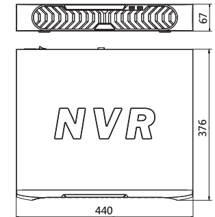
Figure 2-1 Dimensions (Unit:mm)
